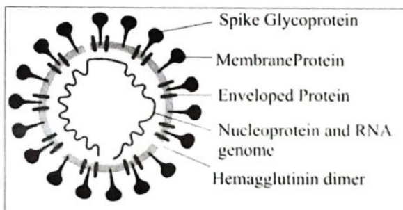
Figure 1: Schematic representation of the coronavirus structure.
